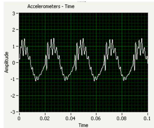
Figure 12 PD Vibration Reading
