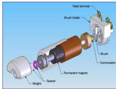
Figure 6 Bar-Type Motor Internal Construction Diagram
