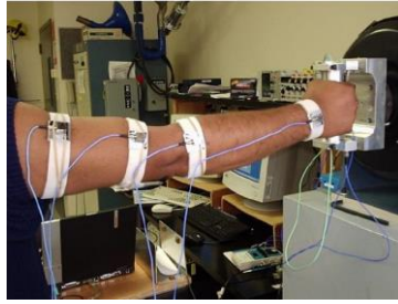
Figure 2 Set-up for Natural Frequency Reading
