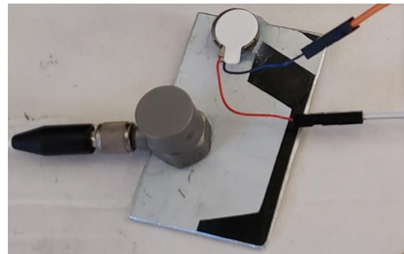
Figure 17 Coin-Type setup
