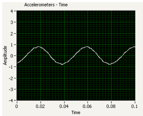
Figure 20 Uxcell Vibration Reading
