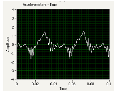
Figure 29 Uxcell Vibration Motor Test
