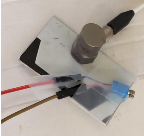
Figure 14 Bar-Type setup
