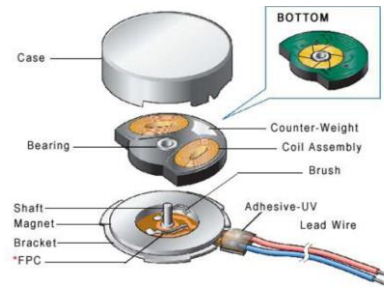
Figure 4 Coin-Type Motor Internal Construction Diagram
