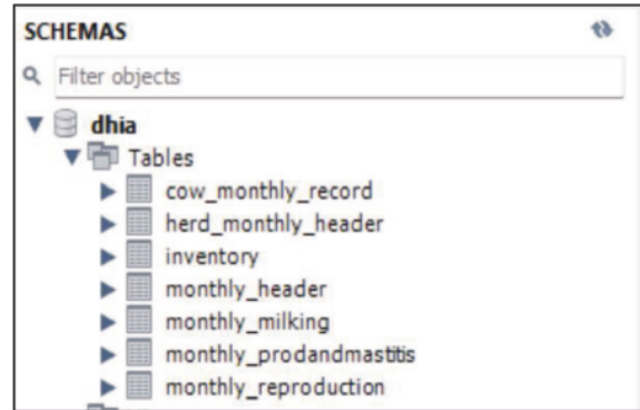
Figure 6 Database tables
