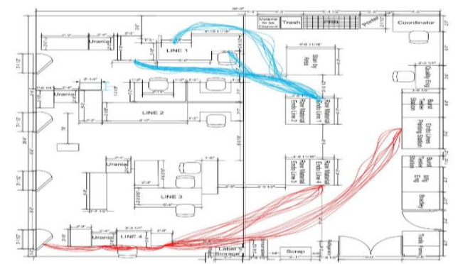
Figure 5 Spaghetti Diagram – Operators Motions
