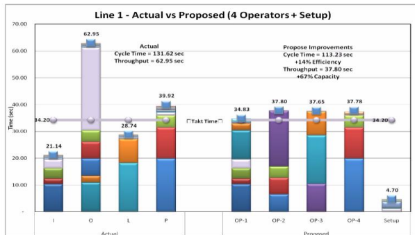
Figure 7 Line Balance Method
