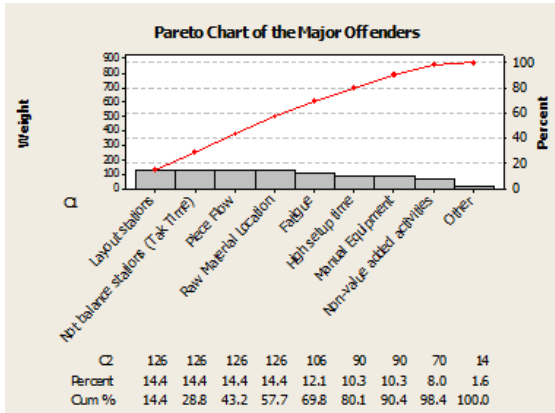
Figure 6 Pareto Chart – Productivity Major Offenders
