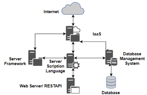
Figure 7 Web Server Infrastructure
