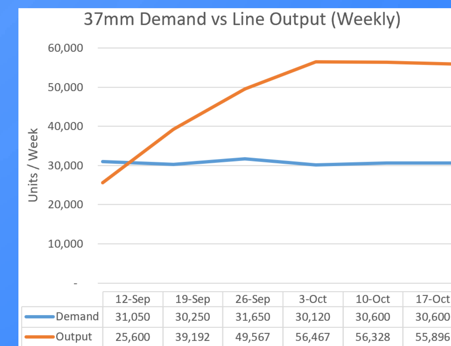
Figure 1 37mm Demand vs Line Output (Weekly)
