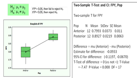
Figure 20 Box Plot
