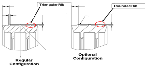
Figure 8 Seal Configurations
