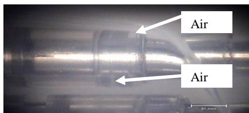
Figure 7 Air Location
