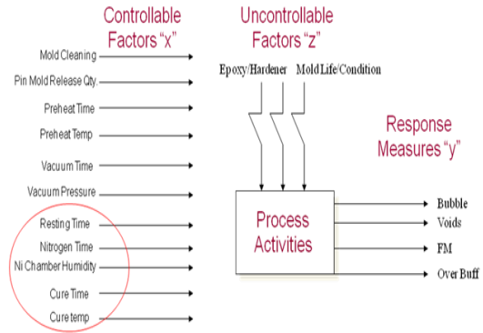
Figure 4 Factors and Response
