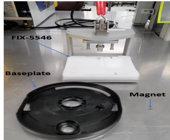
Figure 2 Inputs for Magnet to Baseplate process
