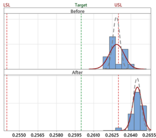
Figure 6 Before and After comparison for the Pocket Diameter dimension
