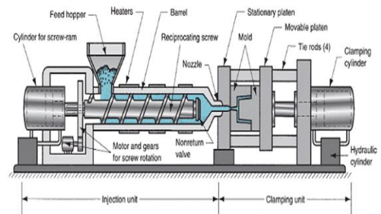
Figure 1 Injection Machine Diagram
