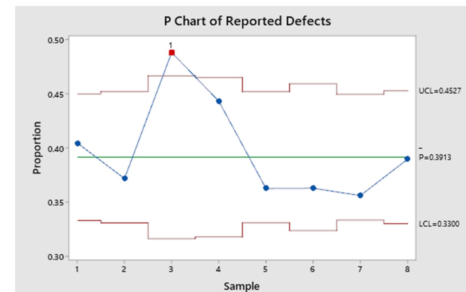
Figure 1 P Chart of Reported Defects
