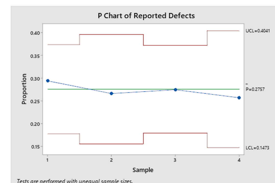
Figure 4 P Chart of Reported Defects with Solution
