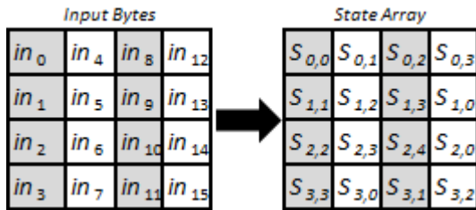
Figure 11 Input Bytes to State Array
