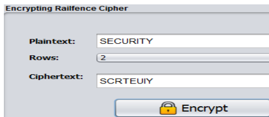
Figure 6 Encryption using the Rail Fence Cipher
