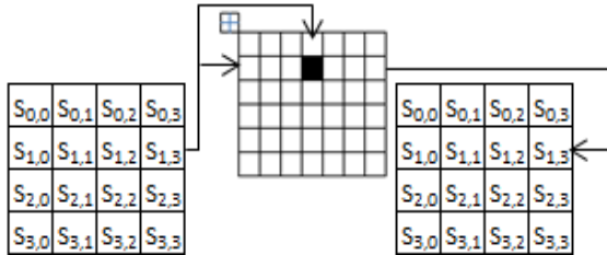
Figure 14 Substitution of Bytes
