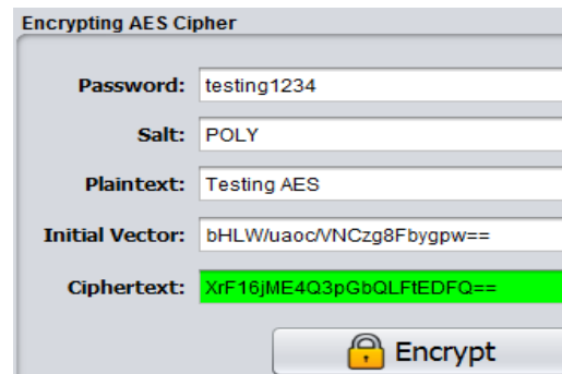
Figure 13 User Input, Encrypting AES
