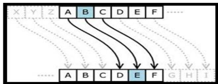
Figure 2 Transformation of the Alphabet
