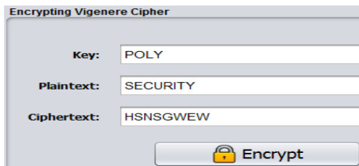
Figure 8 Encrypting a Message using the Vigenere Cipher
