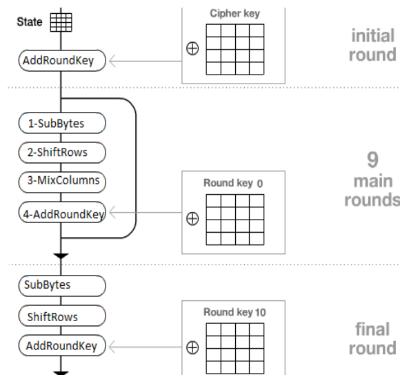
Figure 12 Encryption Process Flowchart
