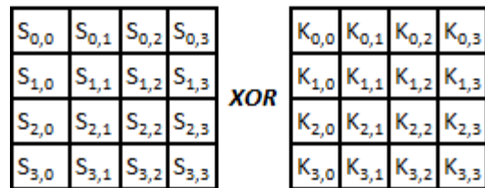
Figure 17 Add Round Key, XOR
